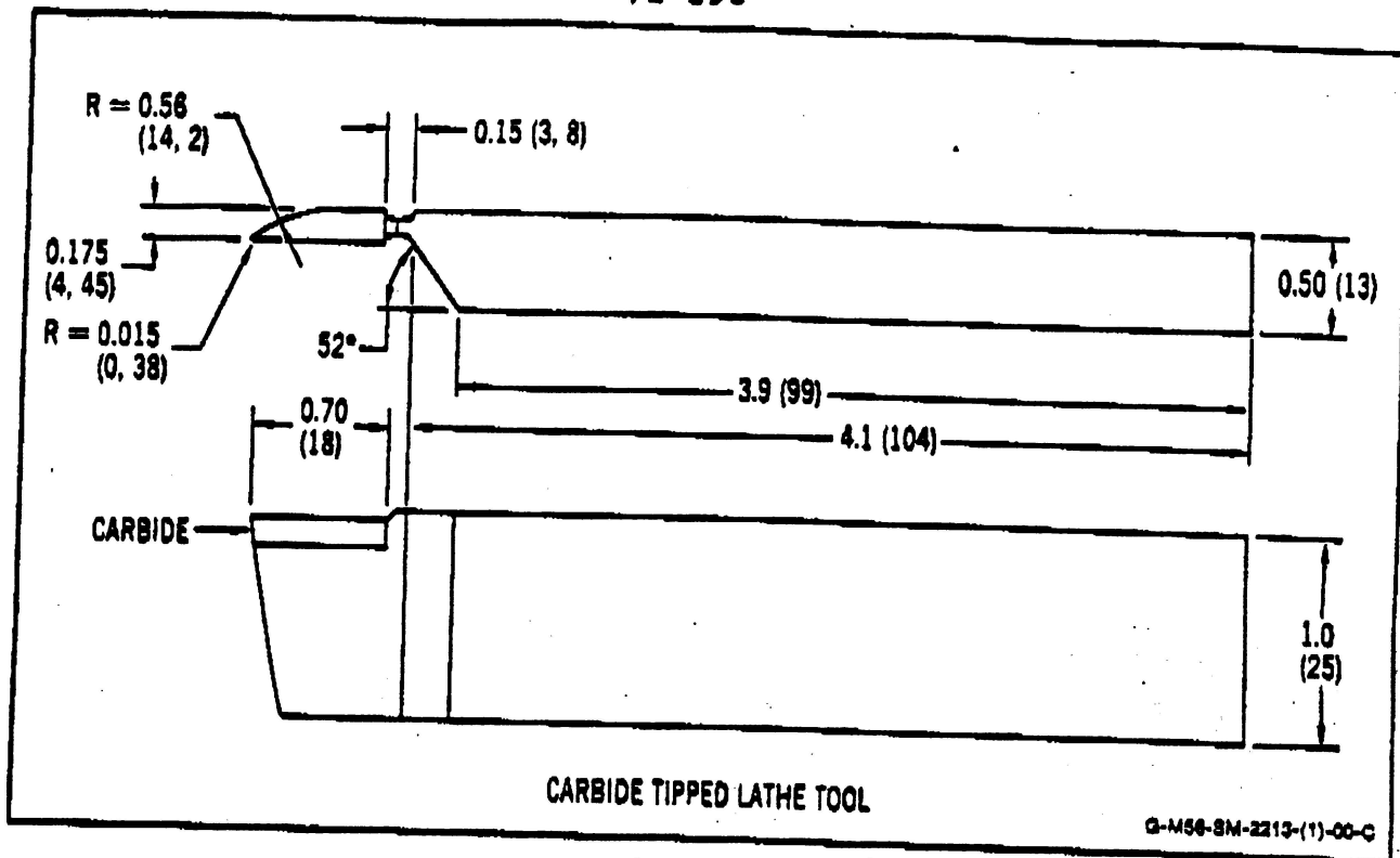
Locally Manufactured Form Tool Figure 902
