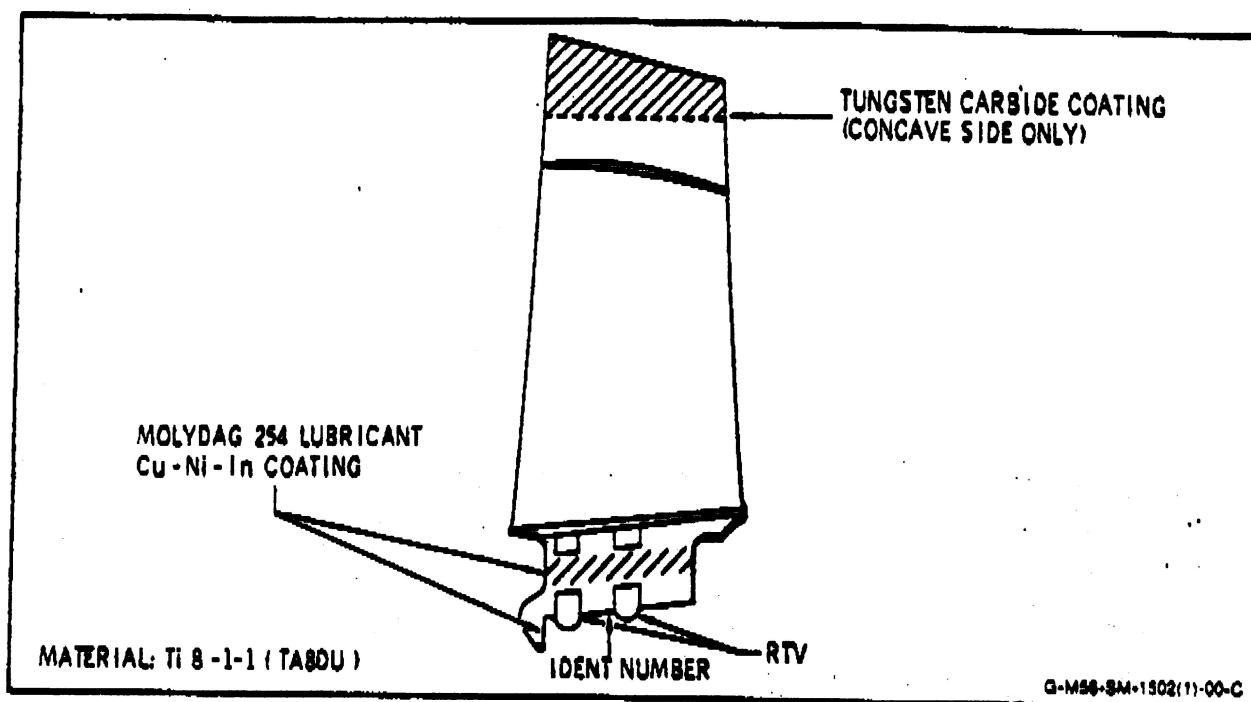
Repair of Compressor Rotor Stage 1 Blades Figure 901
